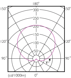
Light Distribution Diagram - EcoHome LEDBulb 12W E27 6500KHV 1PF/20AR
